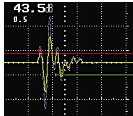
A-scan comparison
